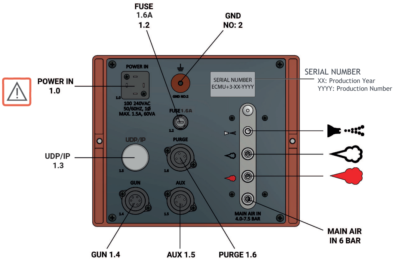
Back Panel Connections
