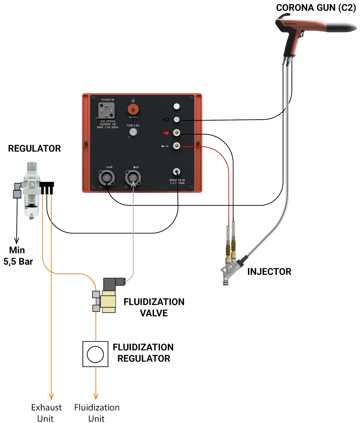
System Connections for E-COAT+3 PRO
